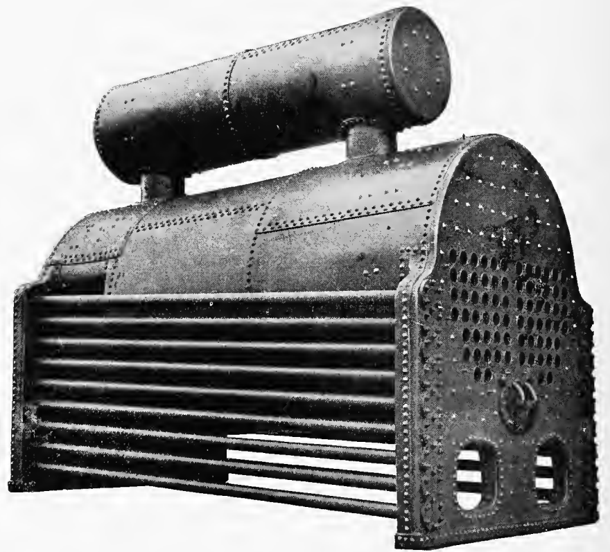
SLOAT'S FIRE AND WATER-TUBE BOILER.
